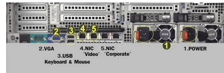
Figure 1 - NVR RAID Server 2U Hardware Connections
